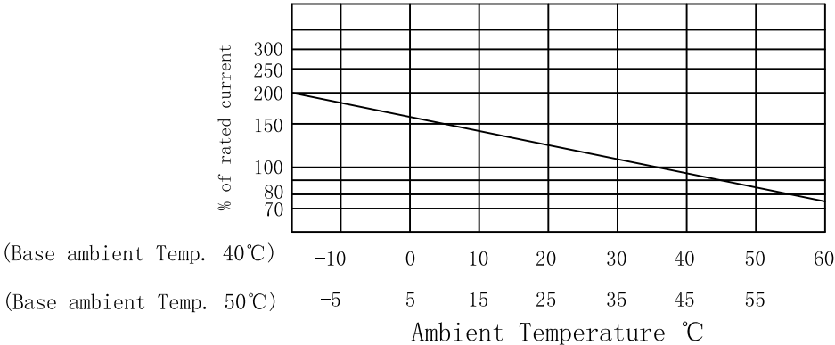
Compensation Curve
