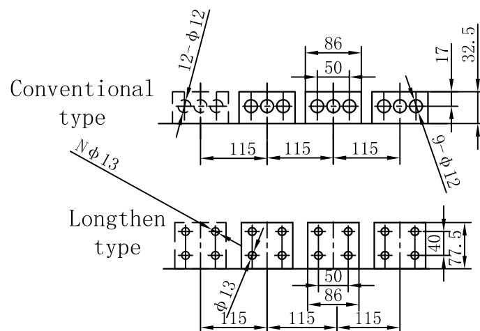
Dimension of fixed type ACB (BW-3200)
