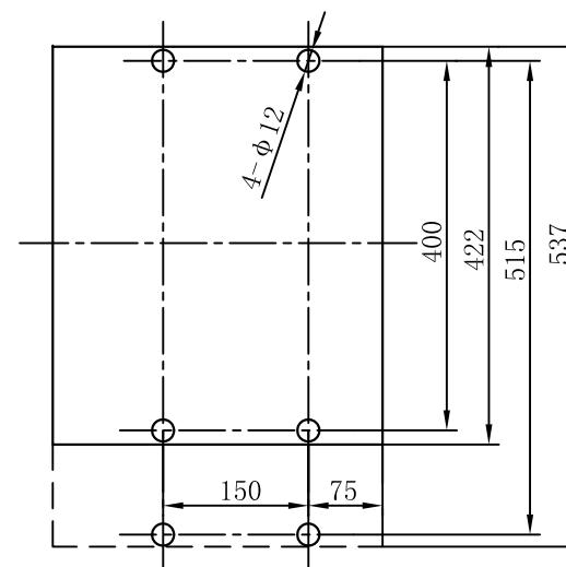
Dimension of fixed type ACB (BW-3200)
