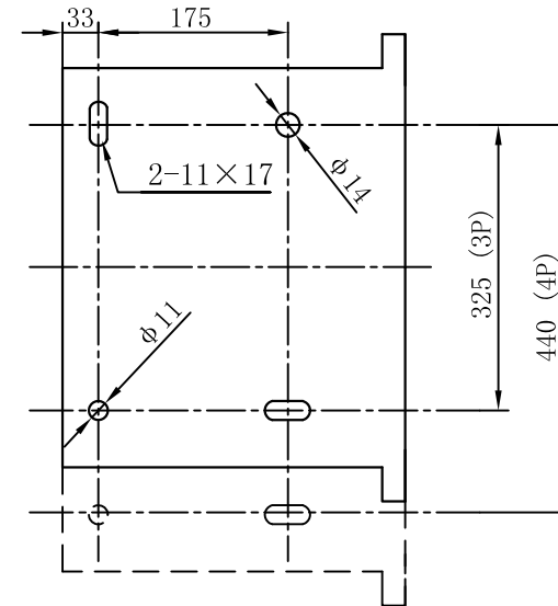
Dimension of drawout type ACB (BW-4000)
